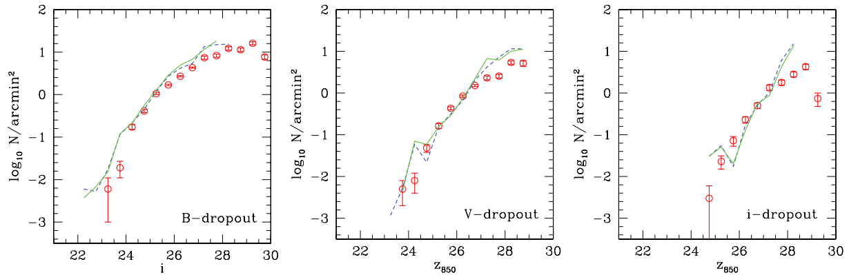
Figure 4. Number counts of B -, V - and i -dropouts. (Red) points are from Bouwens et al. (2007), the (blue) dashed and (green) solid lines give the predictions of the two best-fitting models, respectively, STD.F090.E01 and STD.F095.E03 .
