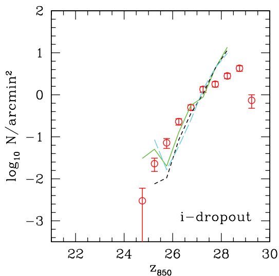
Figure 5. Number counts of i -dropouts. (Red) points are from Bouwens et al. (2007), the (green) solid line gives the predictions of the best-fitting model STD.F095.E03 , the (black) dashed and the (cyan) long-dashed lines correspond to the same combination of parameters but with the contribution of \text{Ly}\alpha emission line in the two different prescription discussed in Section 2.4 (black: STD.F095.E03.LYA1 , cyan: STD.F095.E03.LYA2 ).
