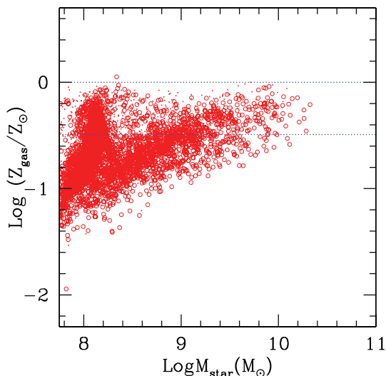
Figure 13. Stellar mass–gas metallicity relation for model galaxies at z = 5 . In this plot, all galaxies in the box are used. Bigger open points refer to central galaxies. The two horizontal lines mark solar and 1/3 solar metallicities. We removed galaxies with less than 10 per cent gas fraction.
