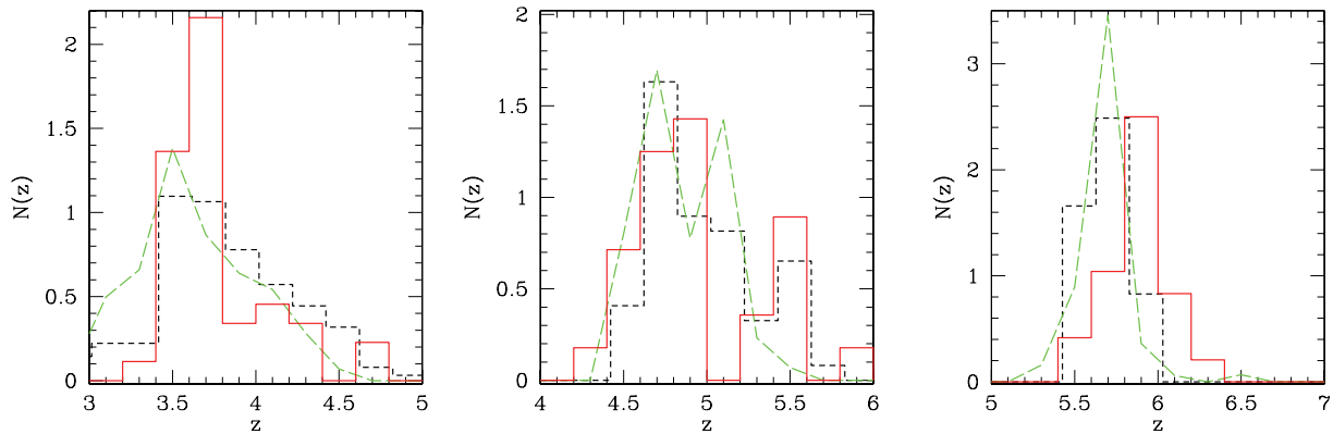
Figure 7. Redshift distribution for B -, V - and i -dropouts in the GOODS-S (red solid lines) and GOODS-MUSIC (black dashed lines) data samples ( z_{850} < 26.2 ) and in the STD.F095.E03 model (green long-dashed lines).
