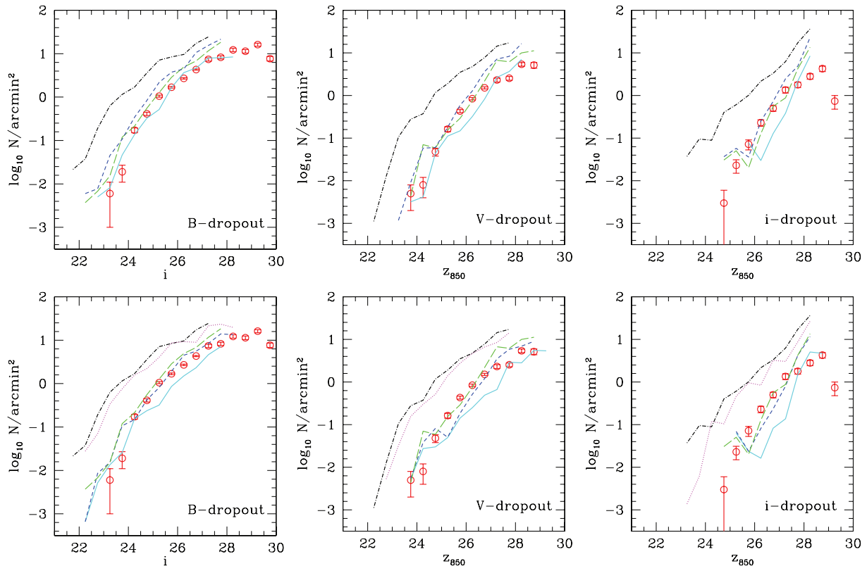
Figure 3. Number counts of B -, V - and i -dropouts. (Red) points are from Bouwens et al. (2007). Upper panels: models with f_{\text{mol}} = 0.95 , \text{STD.F095.E10} (cyan solid lines), \text{STD.F095.E03} (green long-dashed lines) and \text{STD.F095.E01} (blue dashed lines) compared to the model without dust attenuation (black dot-dashed lines). Lower panels: models with t_{\text{esc}} = 0.3 , \text{STD.F050.E03} (cyan solid lines), \text{STD.F090.E03} (blue dashed lines) and \text{STD.F095.E03} (green long-dashed lines) and \text{STD.F100.E03} (magenta dotted lines) also compared to the model without dust attenuation (black dot-dashed lines).
