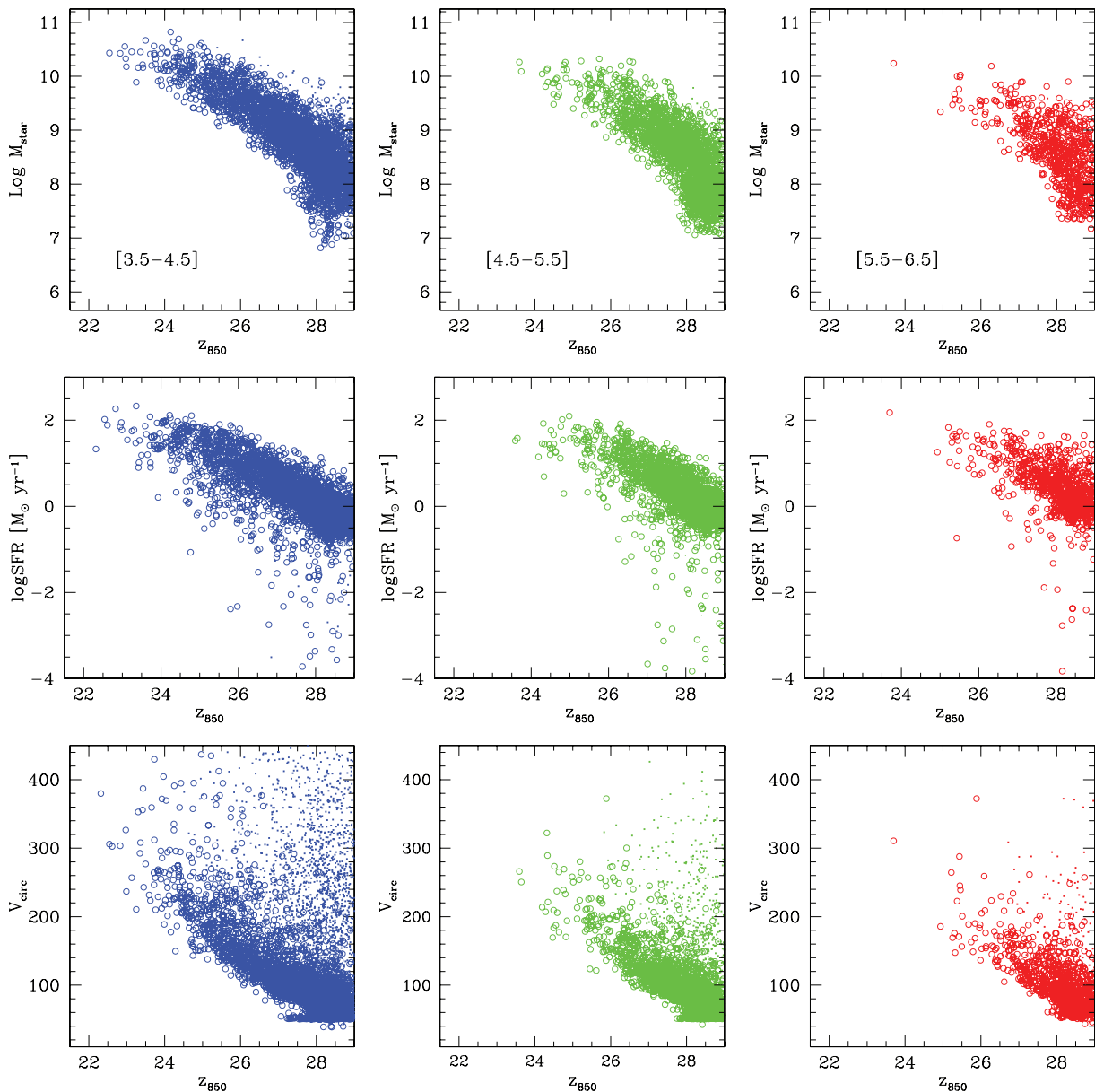
Figure 11. Properties of model Lyman-break galaxies as a function of z_{850} magnitude, for the model STD.F095.E03 . Upper panels give stellar masses, middle panel give star formation rates, lower panels give dark matter halo circular velocities. Bigger open points refer to central galaxies.
