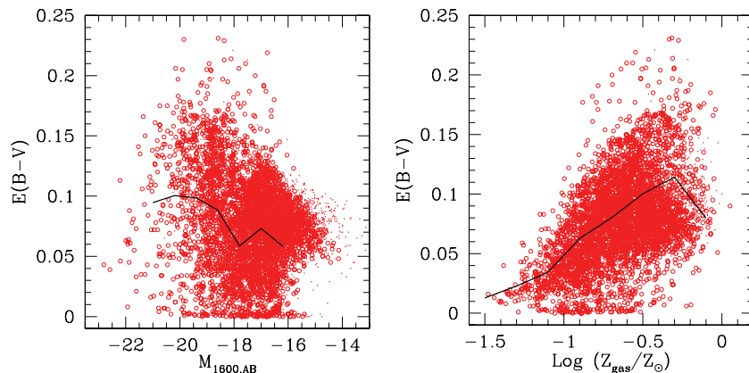
Figure 10. E(B - V) attenuation as a function of the UV rest-frame luminosity M_{1600,AB} (left-hand panel) and gas-metallicity (referred to solar metallicity)(right-hand panel). All model V -dropout galaxies at redshift about 5 and with \log(M_{\star}) > 7.75 are here considered. Open circles refer to central galaxies. The black solid lines represent the ‘weighted’ mean values of E(B - V) computed, respectively, for each bin of magnitude and gas metallicity. B - and i -dropouts show a similar trend.
