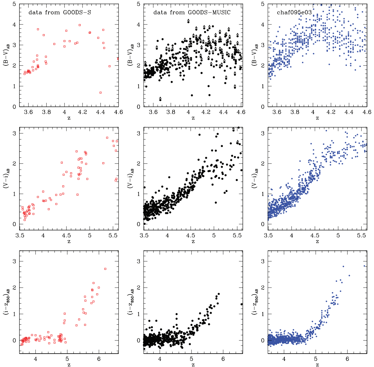
Figure 6. B - V , V - i and i - z_{850} colours of galaxies with z_{850} < 26.2 as a function of redshift. Left-hand panels: GOODS-S galaxies with spectroscopic redshift. Middle panels: GOODS-MUSIC galaxies with photometric redshifts. Black arrows indicate that the magnitude estimation is based on an upper limit at 1\sigma . Right-hand panels: model galaxies (STD.F095.E03).
