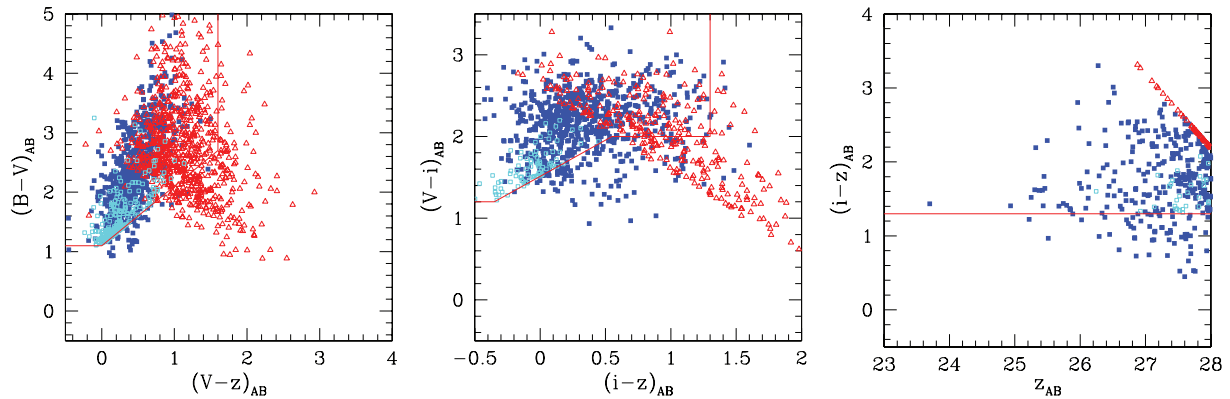
Figure 1. Colour–colour diagrams of B -, V - and i -dropouts for the STD.F095.E03 model. (Blue) filled squares are galaxies with redshift in the specific interval of the selection, i.e. [3.5–4.5], [4.5–5.5] and [5.5–6.5] for B -, V - and i -dropouts, respectively. The open (cyan) squares represent the interlopers (see the text for details), while the (red) open triangles are upper limits in B , V and i . For sake of clarity, only the central galaxies (see Section 2.1) are here considered (satellite galaxies have very similar colours).
