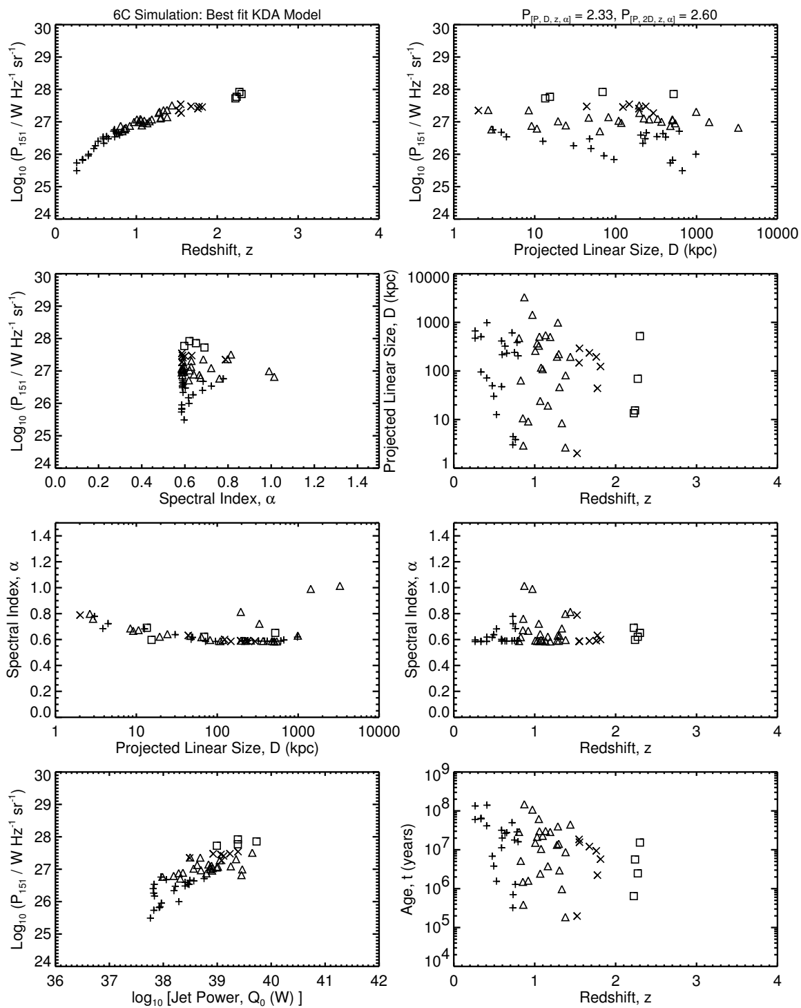
Figure 4.5b: The [P-D-z-\alpha] planes for the 6C simulations of the best fit KDA model, which is the same as in Figure 4.5a. Compare to Figure 3.1b.
