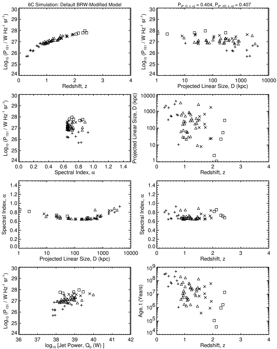
Figure 5.5b: The [P-D-z-\alpha] planes for the 6C simulations of the default BRW-modified model, which is the same as in Figure 5.5a. Compare to Figure 3.1b.
