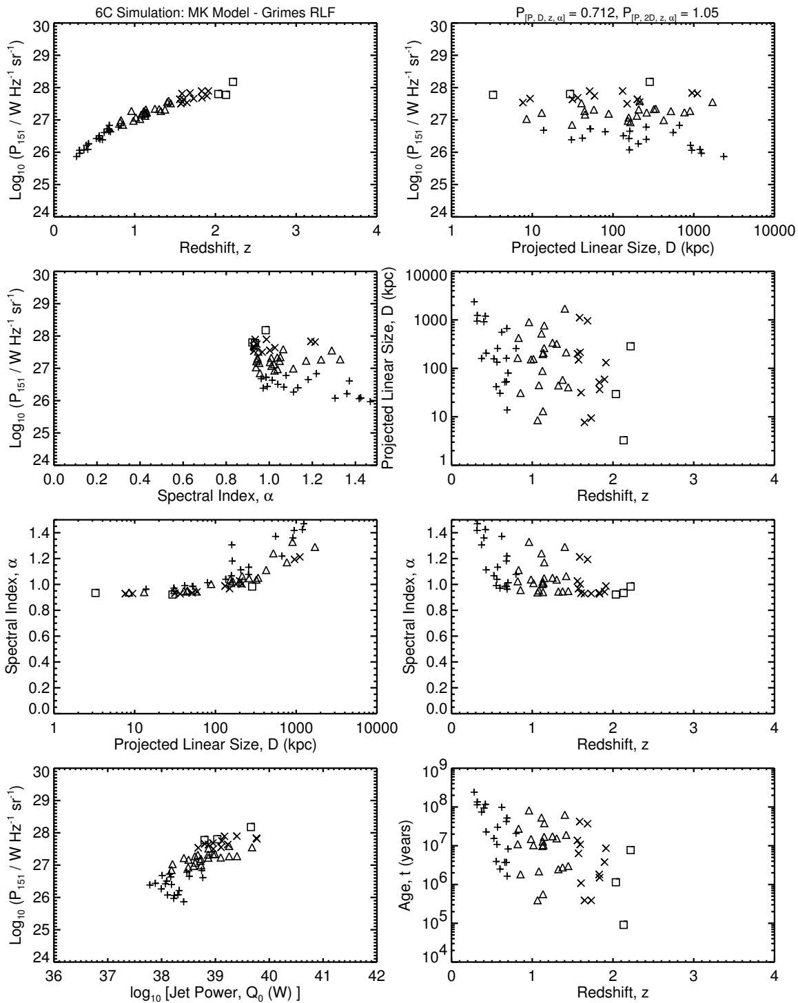
Figure 6.6b: The [P-D-z-\alpha] planes for the 6C simulations of the default MK model using Grimes et al. (2004) RLF, which is the same as in Figure 6.6a. Compare to Figure 3.1b.
