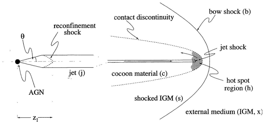
Figure 1.4: Schematic of the basic components of a radio galaxy. Copied from Figure 1 of Kaiser & Alexander (1997), the KDA model (described in Section 2.4 of this thesis).
