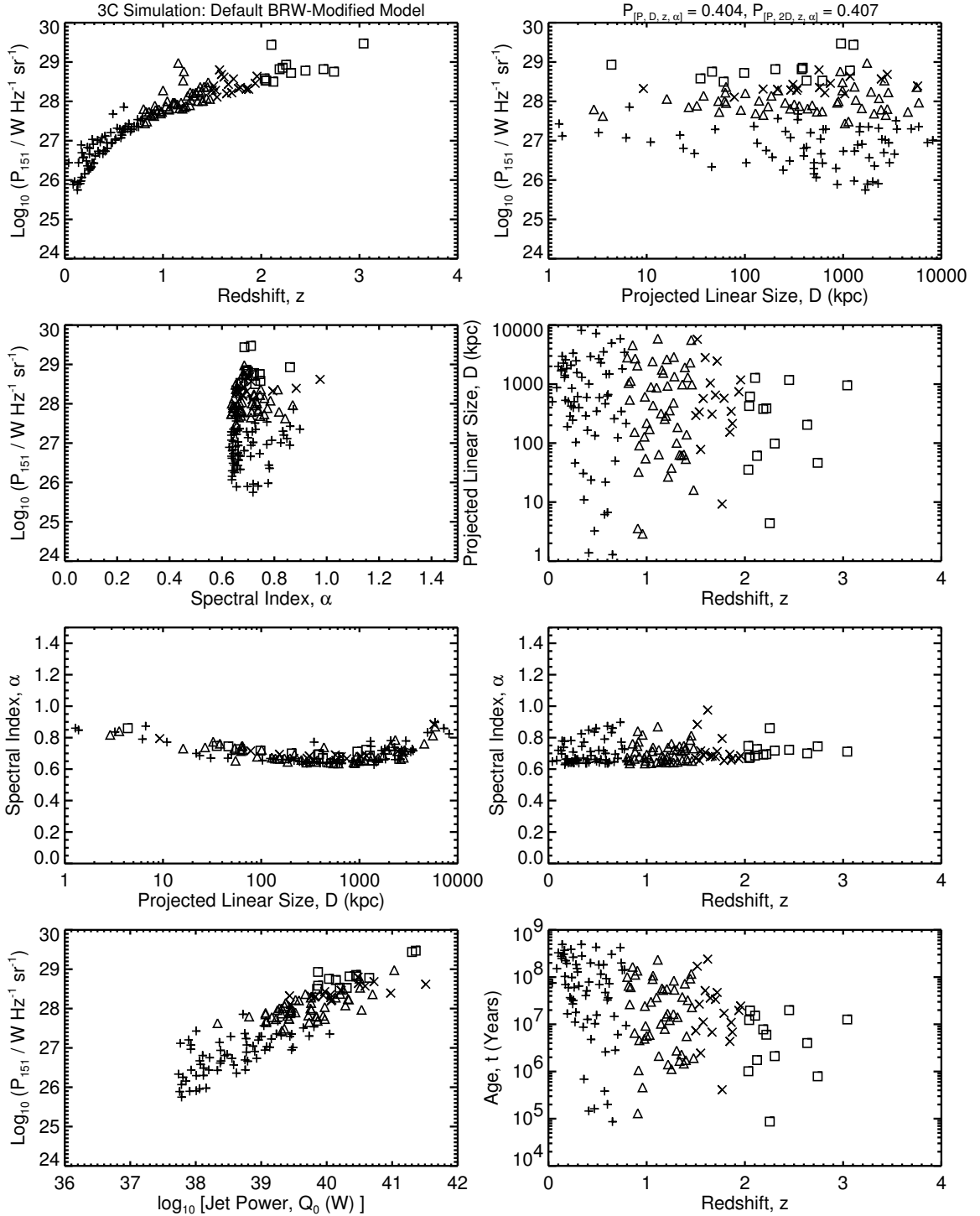
Figure 5.5a: The [P-D-z-\alpha] planes for the 3C simulations of the default BRW-modified model. The initial ensemble (of size 4397469) is generated using x = 2.6 , T_{MaxAge} = 500 Myr; the power evolution is with parameter values as used by the authors in the BRW model, with the hotspot growing in size according to Section 5.2. The 1-D K-S statistics for this case are in the first entry of Table 5.2. Compare to Figure 3.1a.
