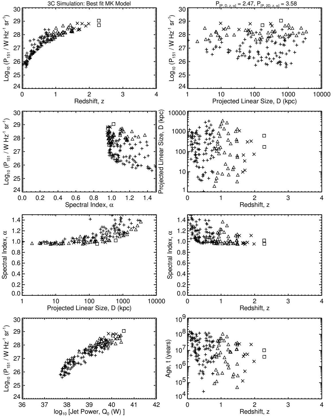
Figure 4.7a: The [P-D-z-\alpha] planes for the 3C simulations of the best fit MK model. The initial ensemble (of size 4861474 – Set 1) is formed using x = 3.0 , T_{MaxAge} = 150 Myr; the power evolution is with parameter variation \gamma_{max} = 3 \times 10^8 , the rest of the parameters having their default values of the MK model. The 1-D K-S statistics for this case are in Table 4.9 (8th row, Run 1) and in Table A.11 (9th entry). Compare to Figure 3.1a.
