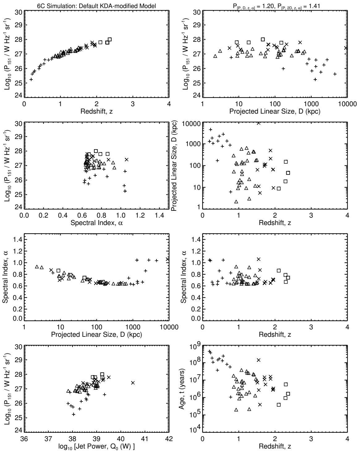
Figure 5.7b: The [P-D-z-\alpha] planes for the 6C simulations of the default KDA-modified. The model is the same as in Figure 5.7a. Compare to Figure 3.1b.
