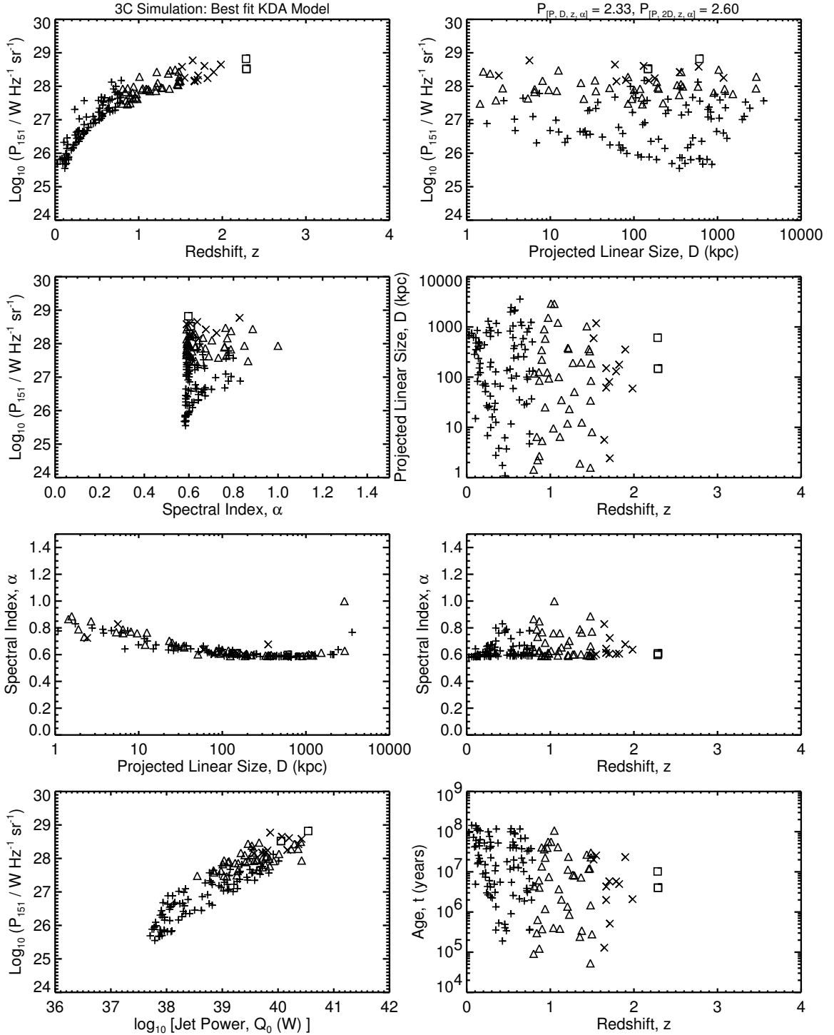
Figure 4.5a: The [P-D-z-\alpha] planes for the 3C simulations of the best fit KDA model. The initial ensemble (of size 4861474 – Set 1) is formed using x = 3.0 , T_{MaxAge} = 150 Myr; the power evolution is with parameter variations \rho_0 = \rho_{0(\text{Default})}/2 and p = 2.12 , the rest being their default values as in the KDA model. The 1-D K-S statistics for this case are in Table 4.7 (8th row, Run 1) and in Table A.1 (14th entry). Compare to Figure 3.1a.
