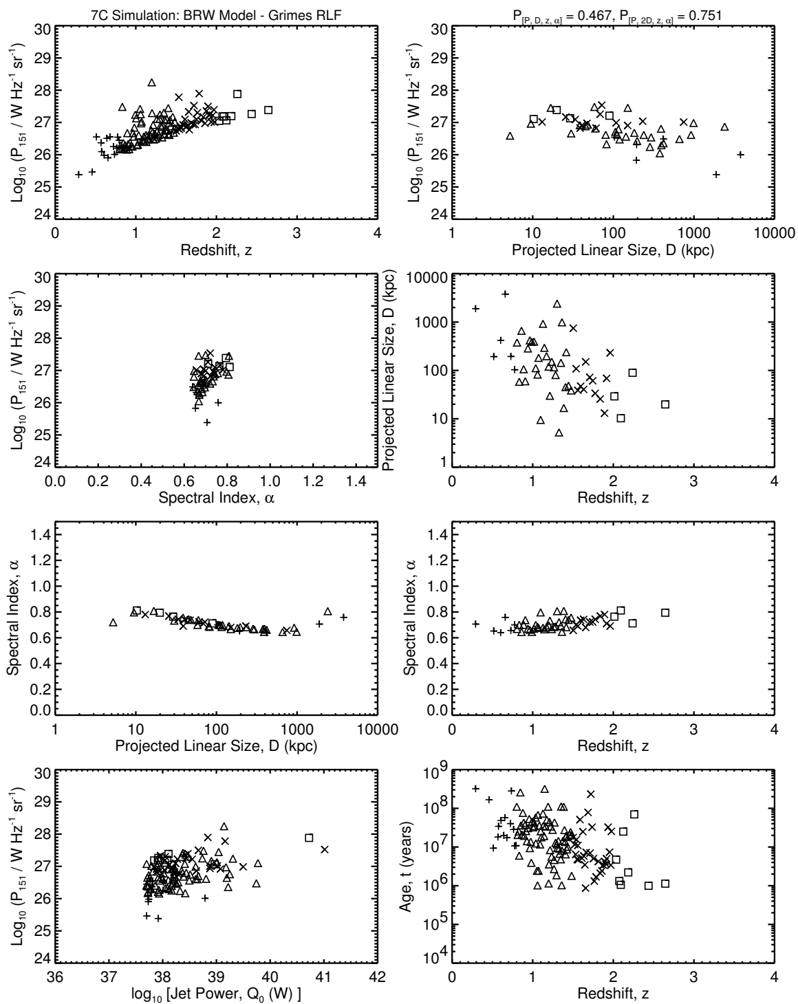
Figure 6.5c: The [P-D-z-\alpha] planes for the 7C simulations of the default BRW model using Grimes et al. (2004) RLF, which is the same as in Figure 6.5a. Compare to Figure 3.1c.
