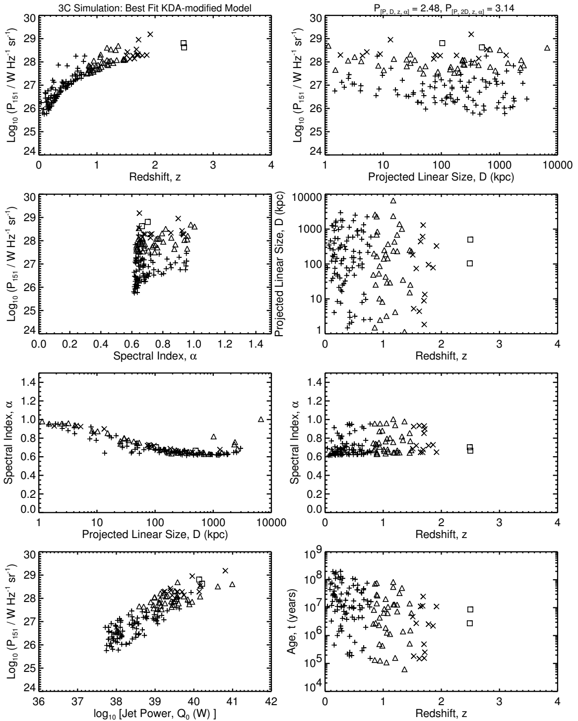
Figure 5.10a: The [P-D-z-\alpha] planes for the 3C simulations of the best fit KDA-modified model. The initial ensemble (of size 4683659) is generated using x = 3.0 , T_{MaxAge} = 200 Myr; the power evolution is with parameter values as used by the authors in the KDA model, with the axial ratio growing in size according to Section 5.3. The 1-D K-S statistics for this case are in Table 5.4 (7th entry). Compare to Figure 3.1a.
