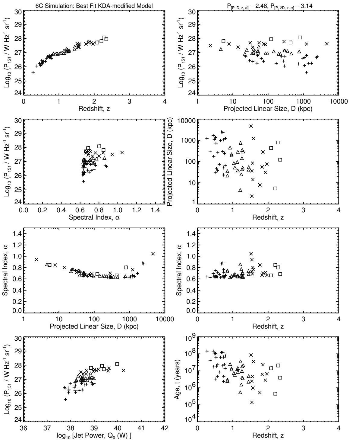
Figure 5.10b: The [P-D-z-\alpha] planes for the 6C simulations of the best fit KDA-modified model, which is the same as in Figure 5.10a. Compare to Figure 3.1b.
