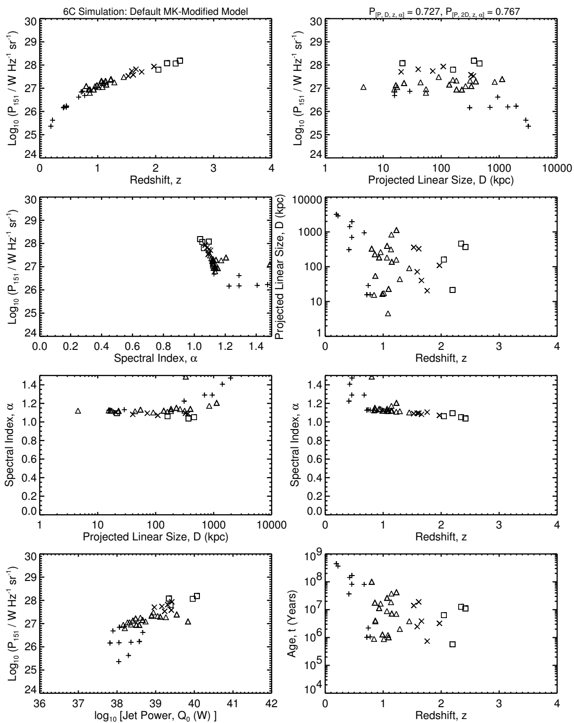
Figure 5.6b: The [P-D-z-\alpha] planes for the 6C simulations of the default MK-modified model, which is the same as in Figure 5.6a. Compare to Figure 3.1b.
