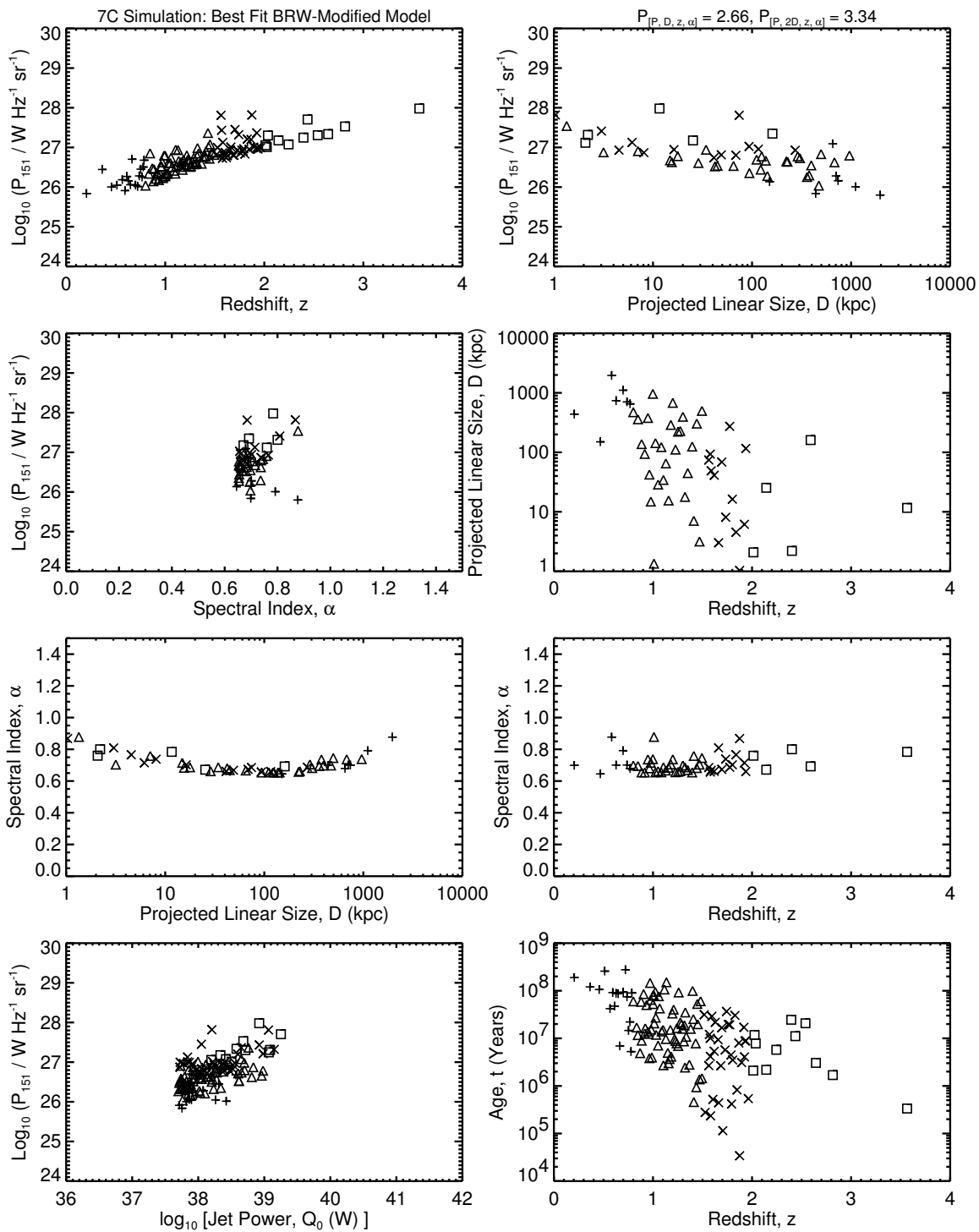
Figure 5.8c: The [P-D-z-\alpha] planes for the 7C simulations of the best fit BRW-modified model, which is the same as in Figure 5.8a. Compare to Figure 3.1c.
