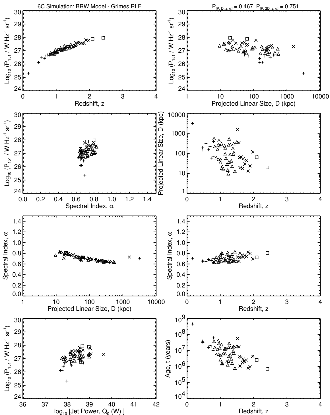
Figure 6.5b: The [P-D-z-\alpha] planes for the 6C simulations of the default BRW model using Grimes et al. (2004) RLF, which is the same as in Figure 6.5a. Compare to Figure 3.1b.
