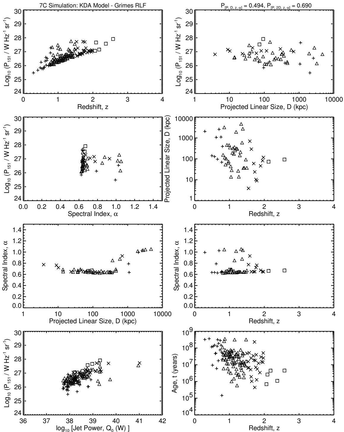
Figure 6.4c: The [P-D-z-\alpha] planes for the 7C simulations of the default KDA using Grimes et al. (2004) RLF. This model is the same as in Figure 6.4a. Compare to Figure 3.1c.
