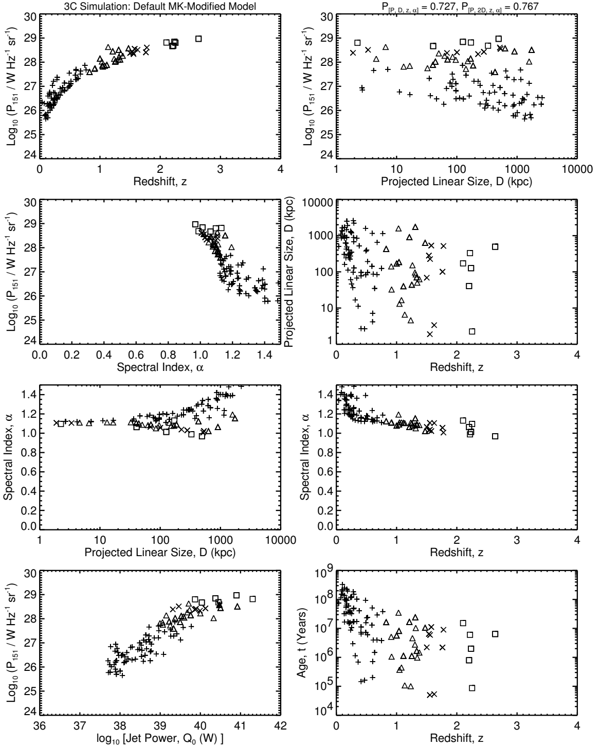
Figure 5.6a: The [P-D-z-\alpha] planes for the 3C simulations of the default MK-modified model. The initial ensemble (of size 4397469) is generated using x = 2.6 , T_{MaxAge} = 500 Myr; the power evolution is with parameter values as used by the authors in the MK model, with the hotspot growing in size according to Section 5.2. The 1-D K-S statistics for this case are in the first entry of Table 5.3. Compare to Figure 3.1a.
