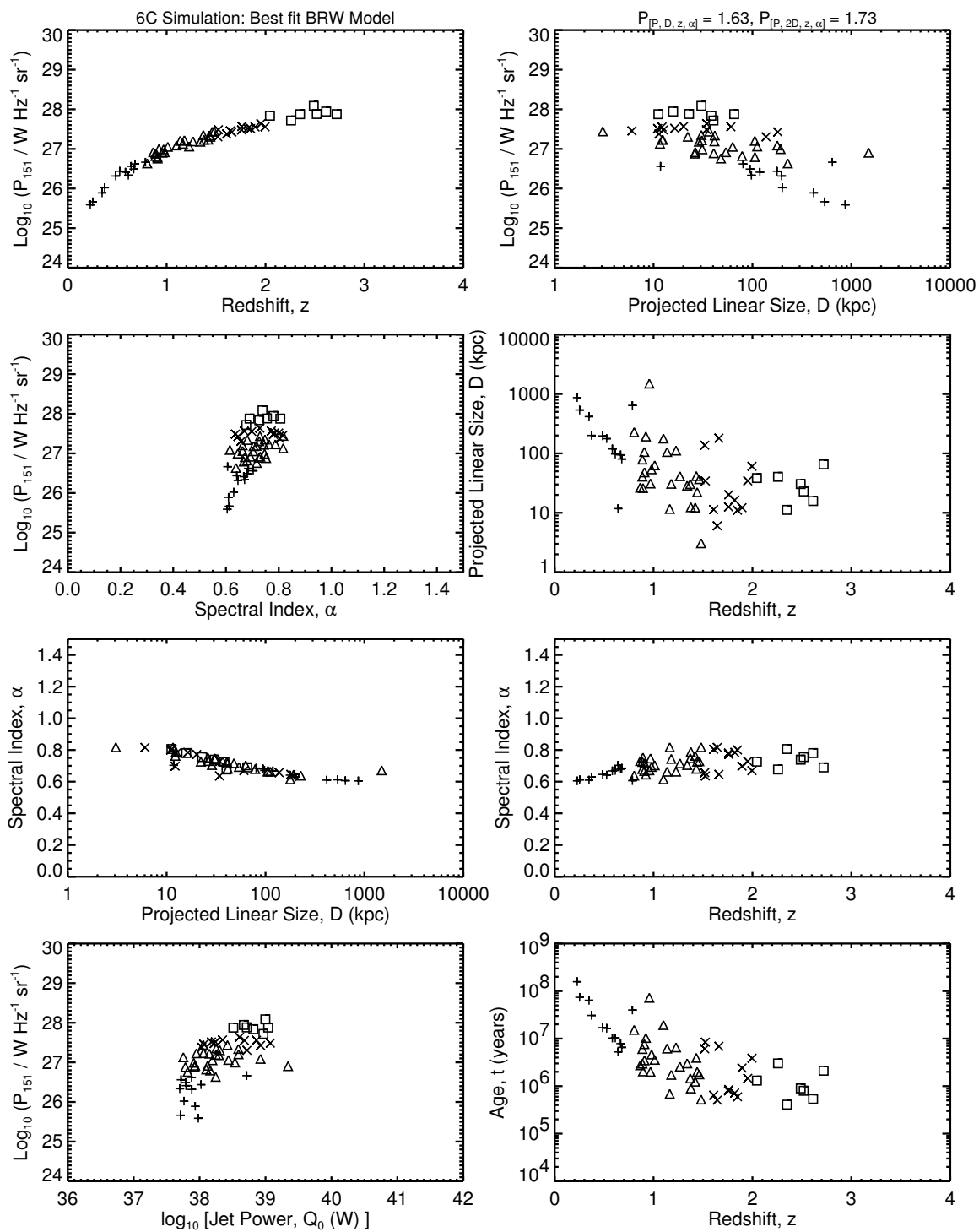
Figure 4.6b: The [P-D-z-\alpha] planes for the 6C simulations of the best fit BRW model, which is the same as in Figure 4.6a. Compare to Figure 3.1b.
