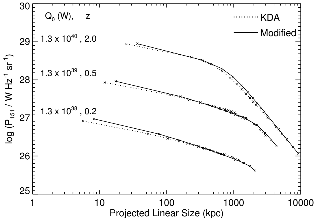
Figure 5.4: [P-D] tracks of three sources with jet powers ( Q_0 ) in Watts and redshifts ( z ) of [1.3 \times 10^{40}, 2.0] , [1.3 \times 10^{39}, 0.5] , [1.3 \times 10^{38}, 0.2] (from top to bottom). Each of the solid and dotted curves correspond to the tracks predicted by the KDA-modified model and the default KDA model, respectively. The crosses on the tracks denote source lifetimes of 1, 10, 20, 30, ..., 90, 100, 150, 200, 250, 300 Myr.
