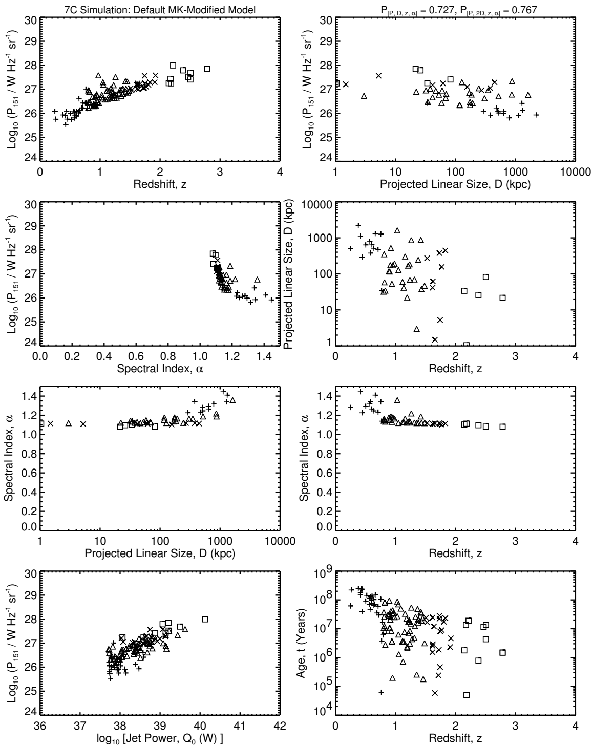
Figure 5.6c: The [P-D-z-\alpha] planes for the 7C simulations of the default MK-modified model, which is the same as in Figure 5.6a. Compare to Figure 3.1c.
