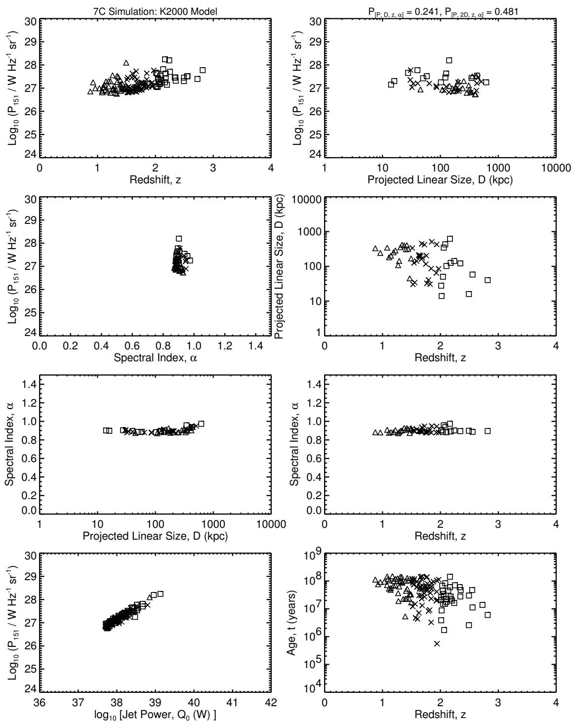
Figure 6.3c: The [P-D-z-\alpha] planes for the 7C simulations of the K2000 model, with parameters as in Figure 6.3a. Compare to Figure 3.1c.
