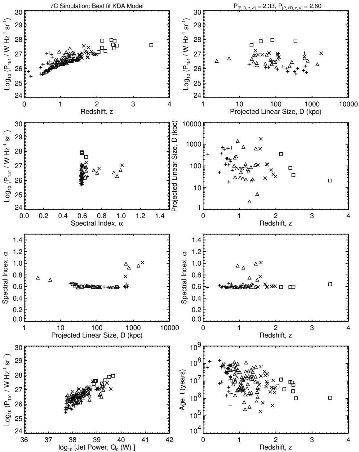
Figure 4.5c: The [P-D-z-\alpha] planes for the 7C simulations of the best fit KDA model, which is the same as in Figure 4.5a. Compare to Figure 3.1c.
