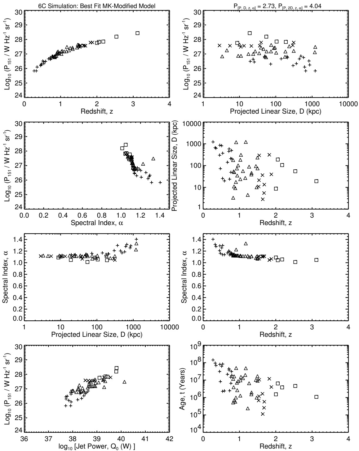
Figure 5.9b: The [P-D-z-\alpha] planes for the 6C simulations of the best fit MK-modified model, which is the same as in Figure 5.9a. Compare to Figure 3.1b.
