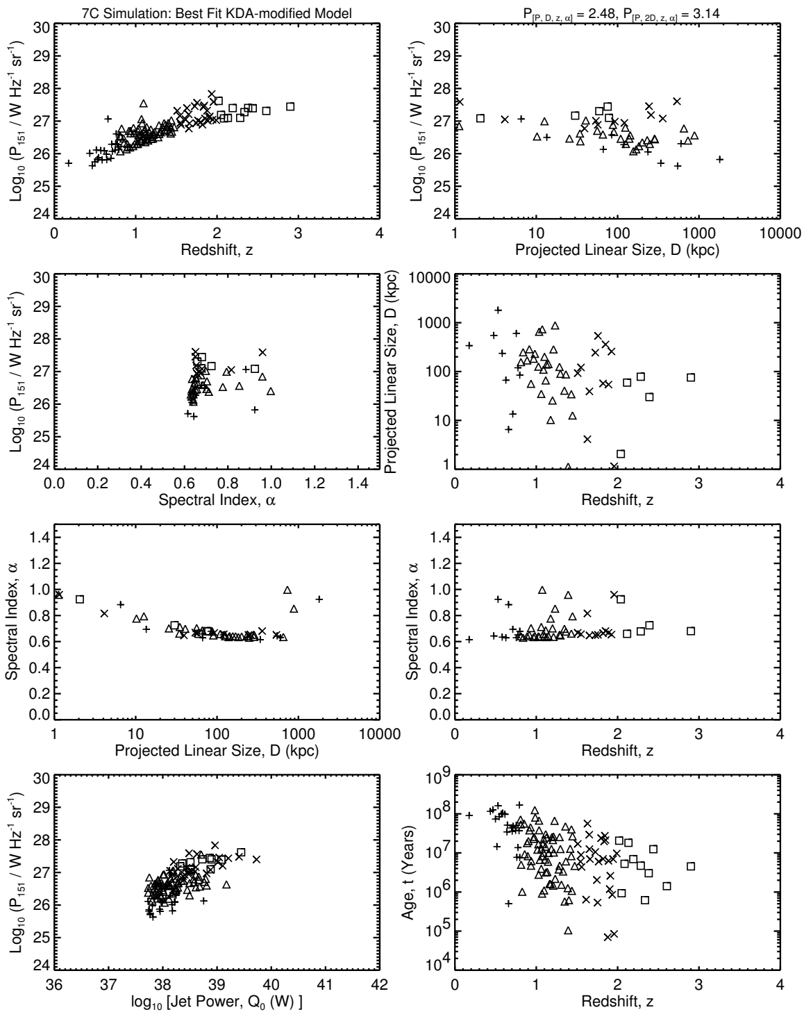
Figure 5.10c: The [P-D-z-\alpha] planes for the 7C simulations of the best fit KDA-modified model, which is the same as in Figure 5.10a. Compare to Figure 3.1c.
