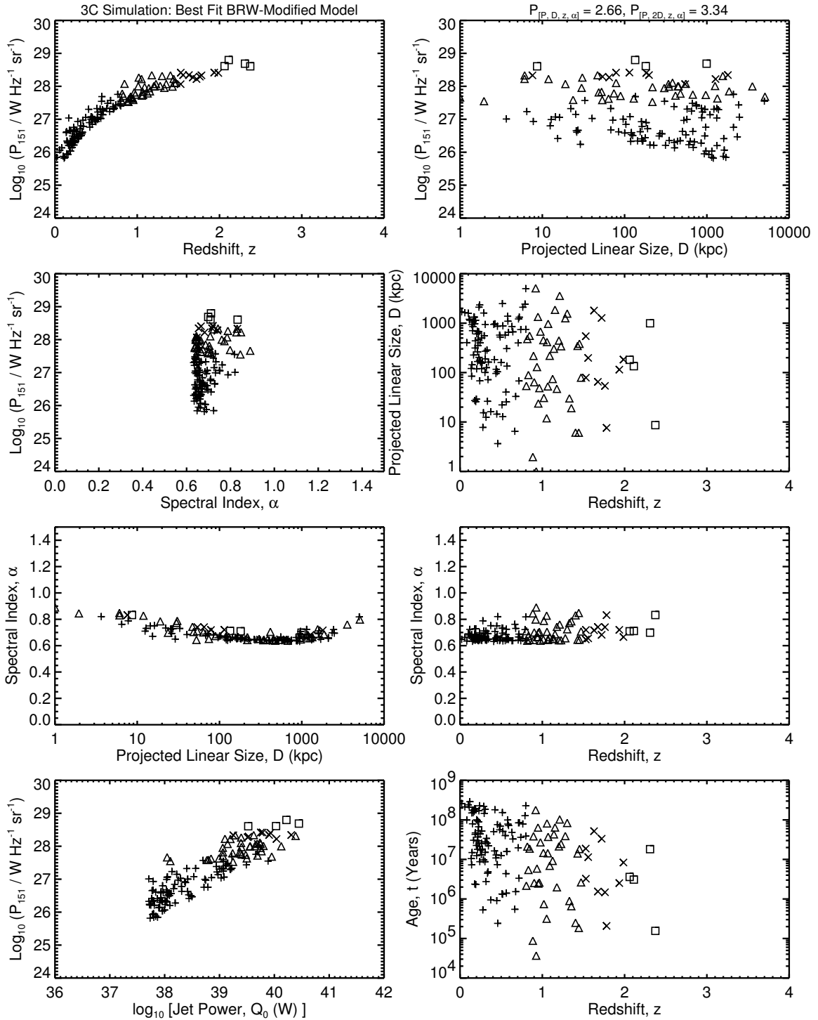
Figure 5.8a: The [P-D-z-\alpha] planes for the 3C simulations of the best-fit BRW-modified model. The initial ensemble (of size 4963343 – Set 4) is generated using x = 3.0 , T_{MaxAge} = 300 Myr; the power evolution is with the parameter variation of t_{bf} = 100 yr, with the rest being their default values as in the BRW-modified model. The 1-D K-S statistics for this case are in Table 5.9 (11th row, Run 4), and in Table B.4 (11th entry). Compare to Figure 3.1a.
