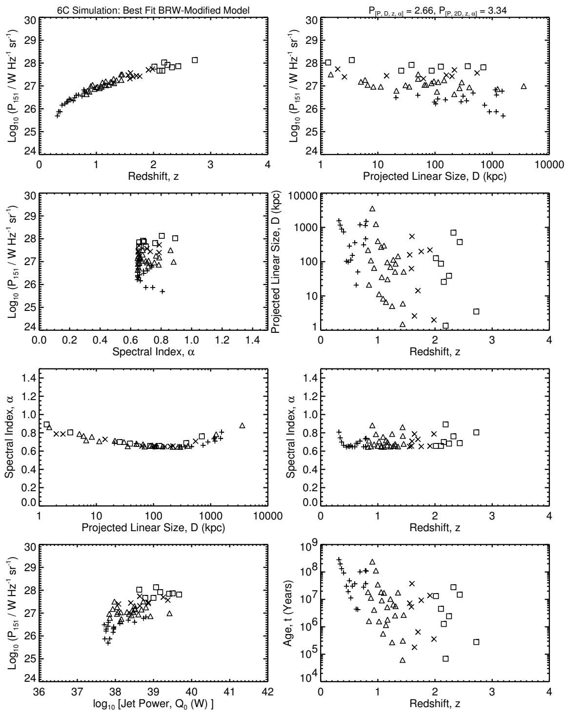
Figure 5.8b: The [P-D-z-\alpha] planes for the 6C simulations of the best fit BRW-modified model, which is the same as in Figure 5.8a. Compare to Figure 3.1b.
