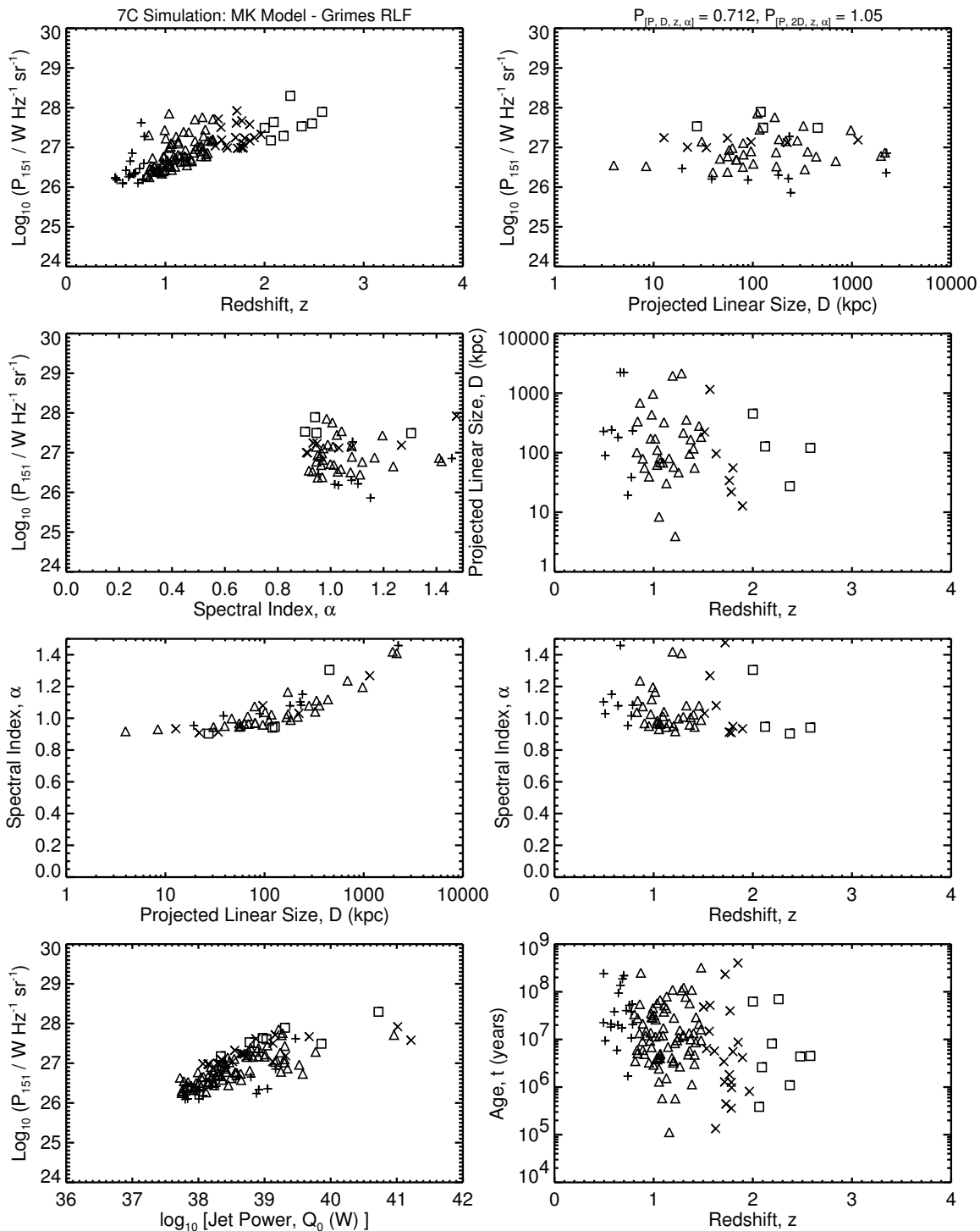
Figure 6.6c: The [P-D-z-\alpha] planes for the 7C simulations of the default MK model using Grimes et al. (2004) RLF, which is the same as in Figure 6.6a. Compare to Figure 3.1c.
