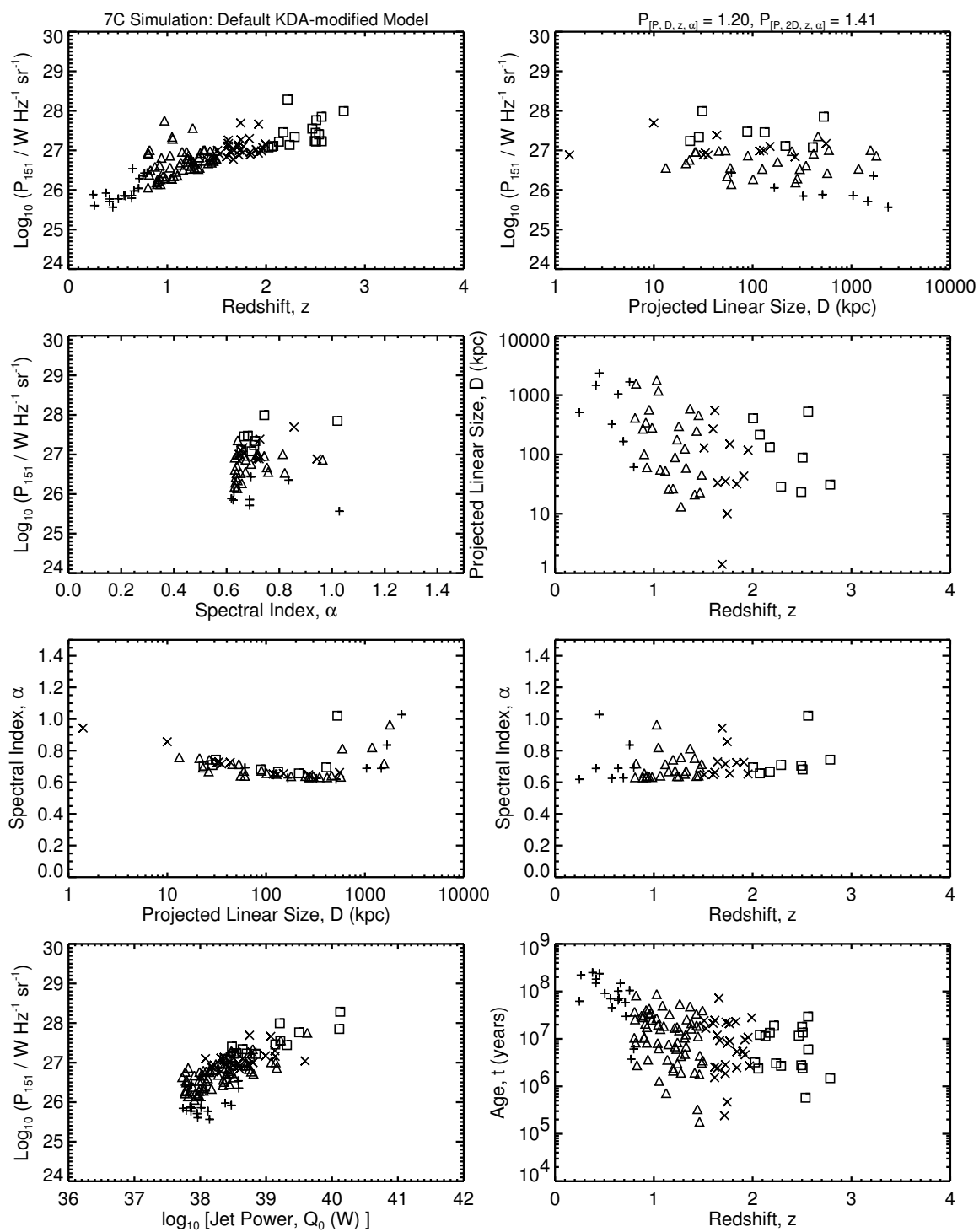
Figure 5.7c: The [P-D-z-\alpha] planes for the 7C simulations of the default KDA-modified. This model is the same as in Figure 5.7a. Compare to Figure 3.1c.
