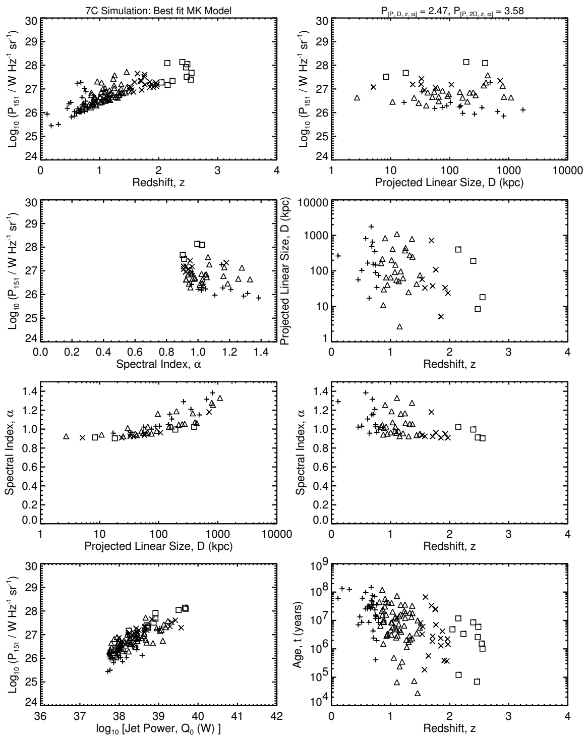
Figure 4.7c: The [P-D-z-\alpha] planes for the 7C simulations of the best fit MK model, which is the same as in Figure 4.7a. Compare to Figure 3.1c.
