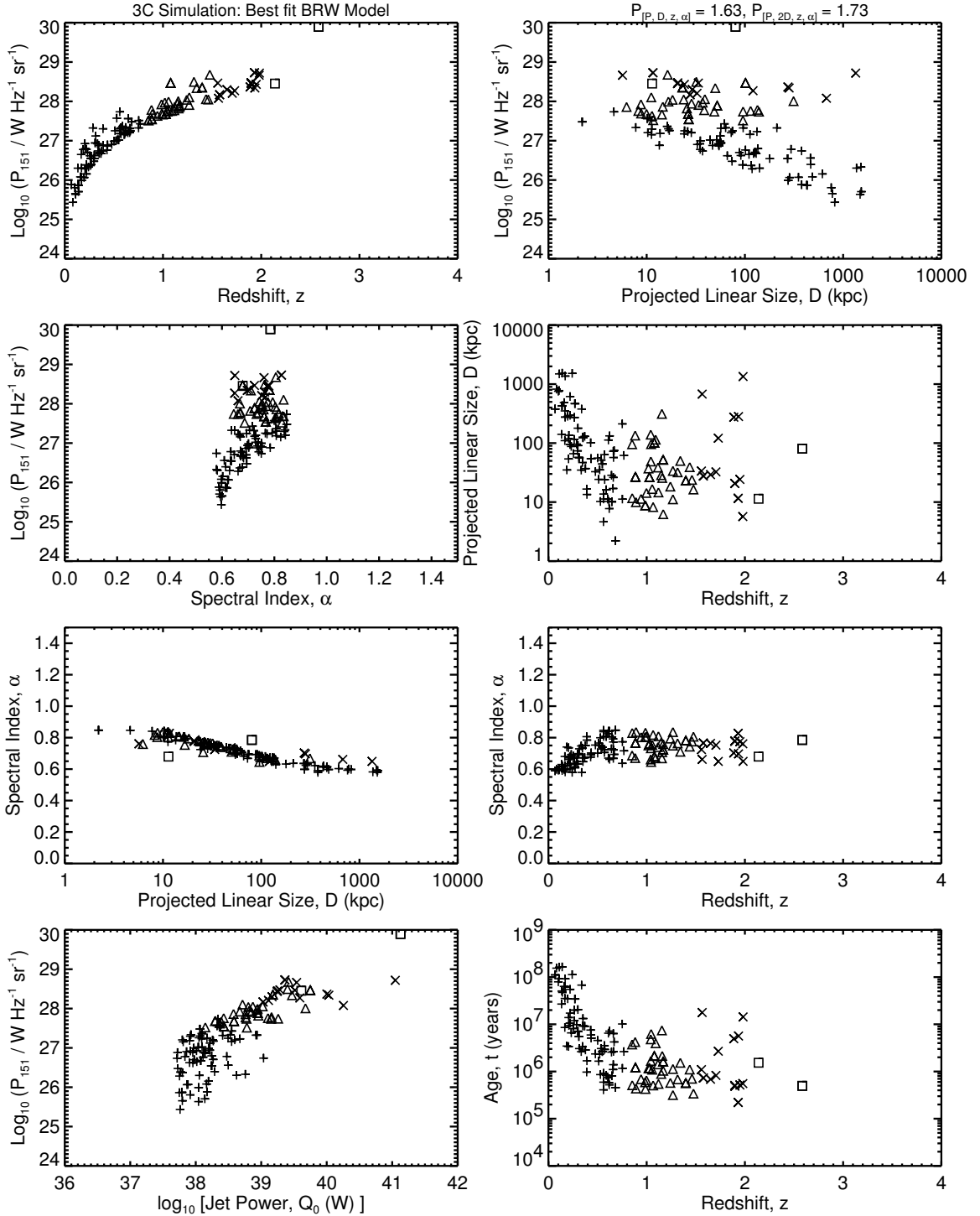
Figure 4.6a: The [P-D-z-\alpha] planes for the 3C simulations of the best fit BRW Model. The initial ensemble (of size 3355926 – Set 3) is formed using x = 3.0 , T_{MaxAge} = 250 Myr; the power evolution is with the parameter variation of a_0 = 7.5 kpc, with the rest being their default values as in the BRW model. The 1-D K-S statistics for this case are in Table 4.8 (2nd row, Run 3) and in Table A.8 (2nd entry). Compare to Figure 3.1a.
