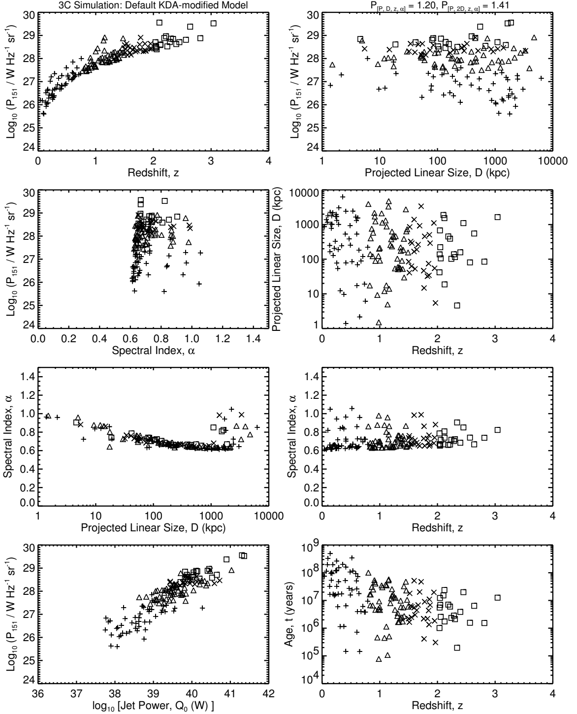
Figure 5.7a: The [P-D-z-\alpha] planes for the 3C simulations of the default KDA-modified model. The initial ensemble (of size 4397469) is generated using x = 2.6 , T_{MaxAge} = 500 Myr; the power evolution is with parameter values as used by the authors in the KDA model, with the axial ratio growing in size according to Section 5.3. The 1-D K-S statistics for this case are in the first entry of Table 5.4. Compare to Figure 3.1a.
