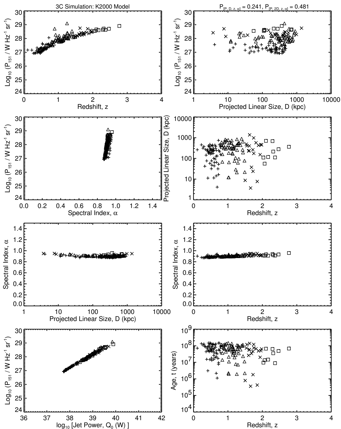
Figure 6.3a: The [P-D-z-\alpha] planes for the 3C simulations of one K2000 model. The initial ensemble (of size 111072) is formed using x = 3.0 , T_{MaxAge} = 150 Myr; the power evolution is with default (fiducial in Table 6.1) parameter values of the K2000 model. The 1-D K-S statistics for this case are in Table 6.2 (3rd model entry from top). Compare to Figure 3.1a.
