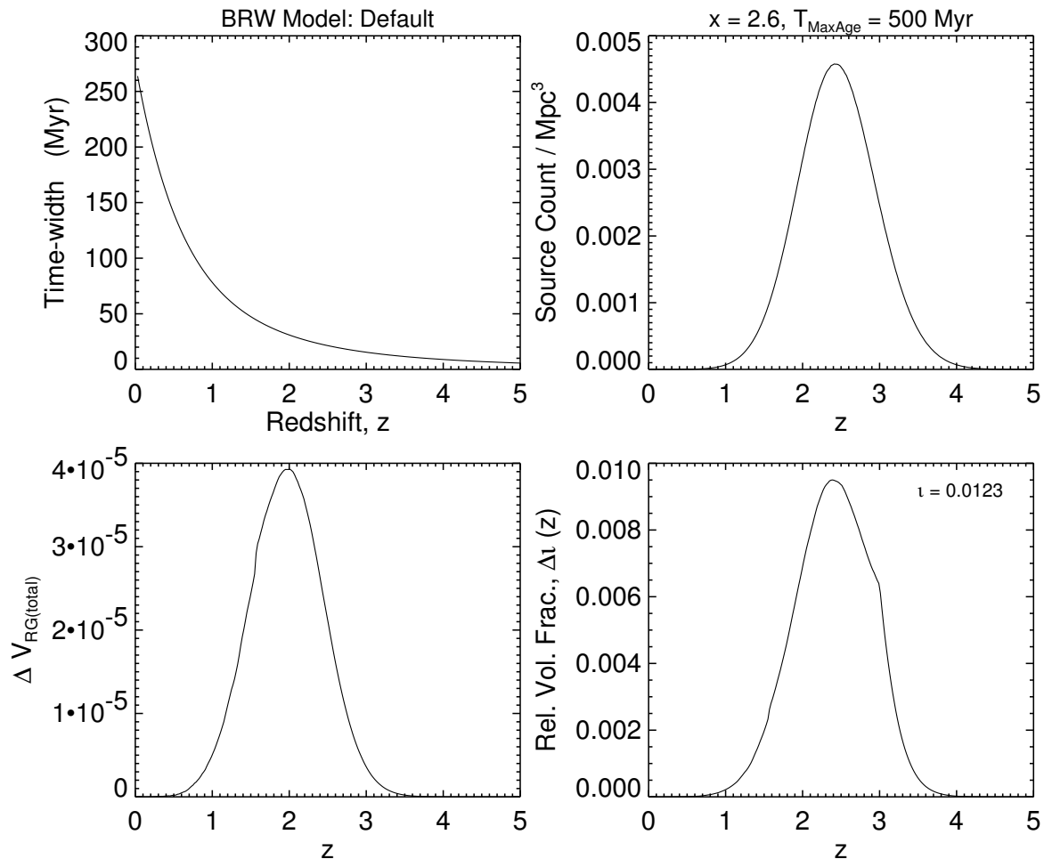
Figure 7.2: Relevant volume fraction of the universe filled by RGs from BRW simulation with default model parameters. The initial ensemble of size 1561417 is generated using x = 2.6 , T_{MaxAge} = 500 Myr. See Section 7.3.2.1 for details.
