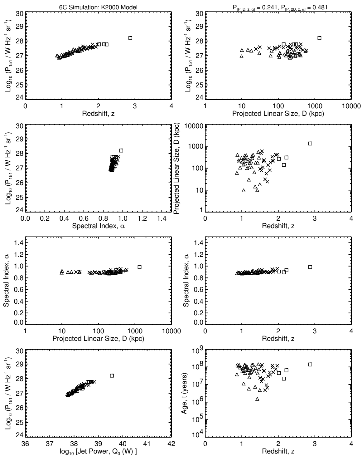
Figure 6.3b: The [P-D-z-\alpha] planes for the 6C simulations of the K2000 model, with parameters as in Figure 6.3a. Compare to Figure 3.1b.
