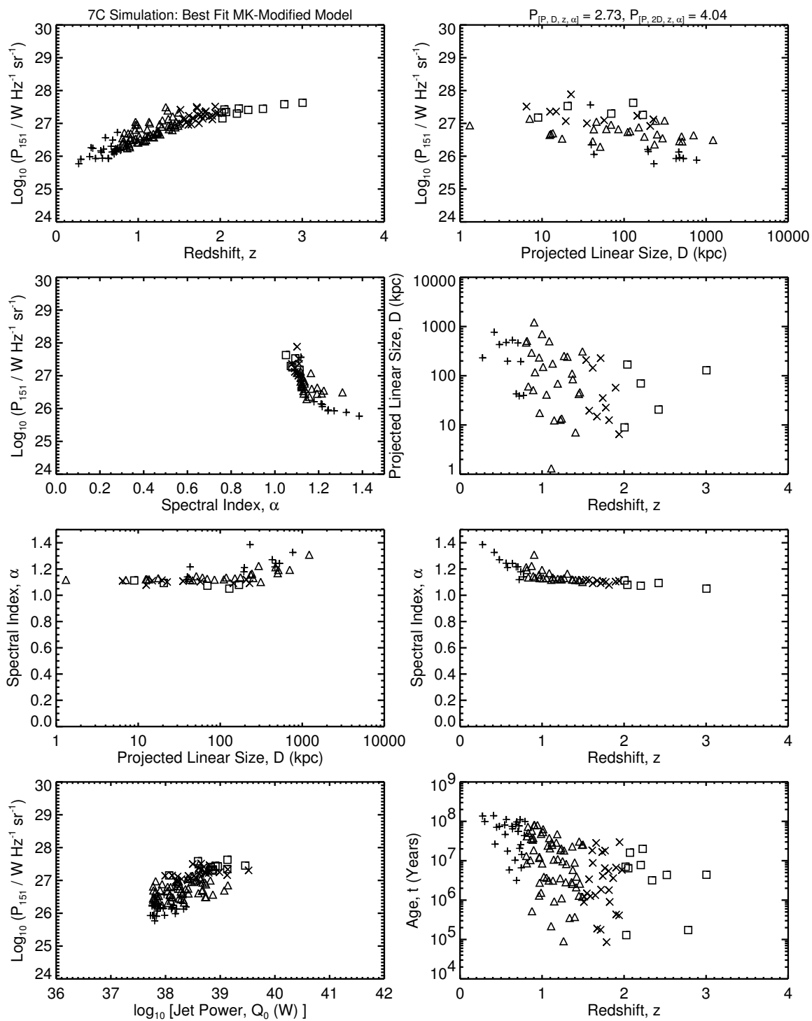
Figure 5.9c: The [P-D-z-\alpha] planes for the 7C simulations of the best fit MK-modified model, which is the same as in Figure 5.9a. Compare to Figure 3.1c.
