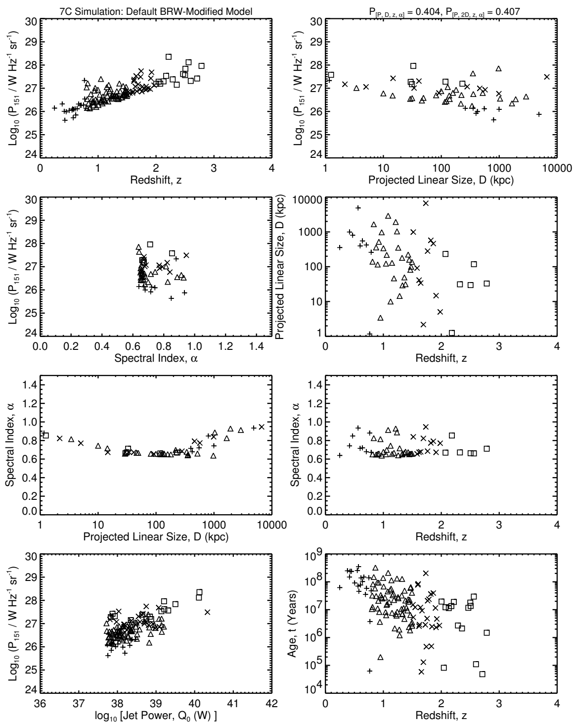
Figure 5.5c: The [P-D-z-\alpha] planes for the 7C simulations of the default BRW-modified model, which is the same as in Figure 5.5a. Compare to Figure 3.1c.
