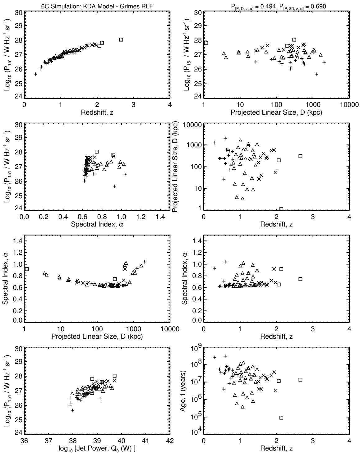
Figure 6.4b: The [P-D-z-\alpha] planes for the 6C simulations of the default KDA using Grimes et al. (2004) RLF. The model is the same as in Figure 6.4a. Compare to Figure 3.1b.
