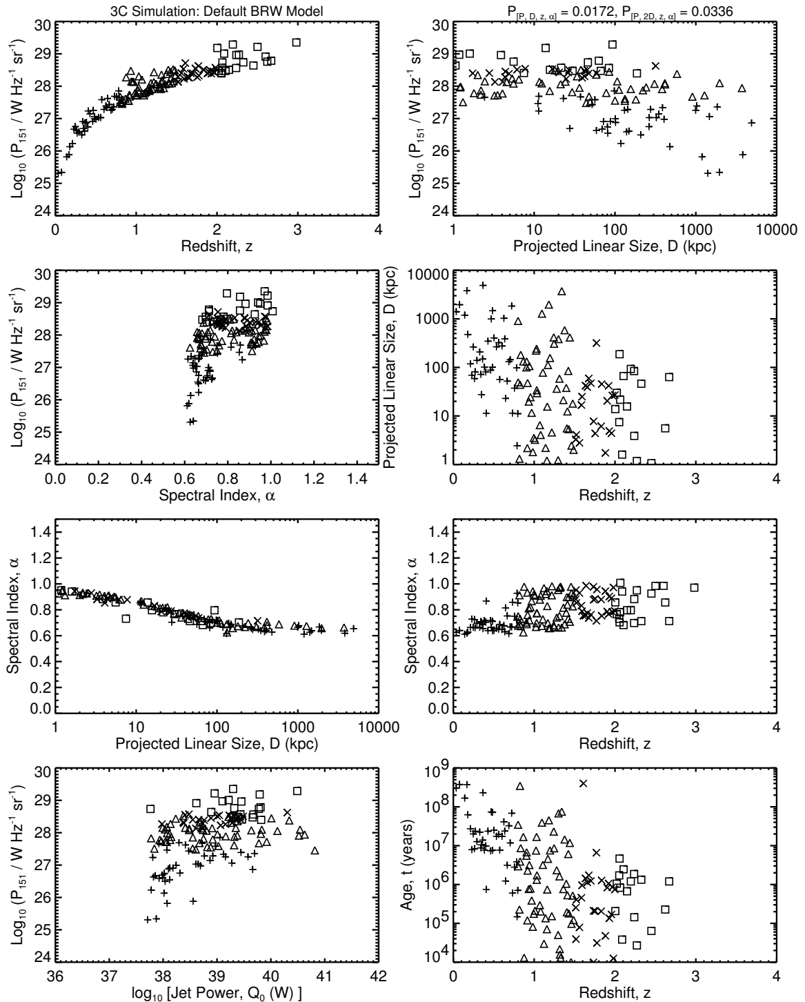
Figure 4.3a: The [P-D-z-\alpha] planes for the 3C simulations of the default BRW model. The initial ensemble (of size 2930490) is formed using x = 2.6 , T_{MaxAge} = 500 Myr; the power evolution is with the default parameter values used in BRW. The 1-D K-S statistics for this case are in the first entry of Table 4.2. Compare to Figure 3.1a.
