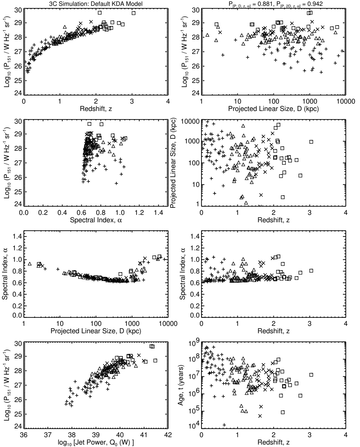
Figure 4.2a: The [P-D-z-\alpha] planes for the 3C simulations of the default KDA model. The initial ensemble (of size 4397469) is formed using x = 2.6 , T_{MaxAge} = 500 Myr; the power evolution is with the default parameter values used in KDA. The 1-D K-S statistics for this case are in the first entry of Table 4.1. Compare to Figure 3.1a.
